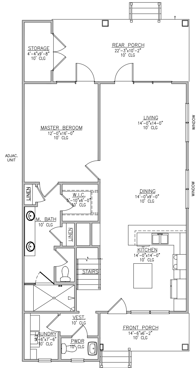
CRANE - 1st FLOOR RIGHT END UNIT
