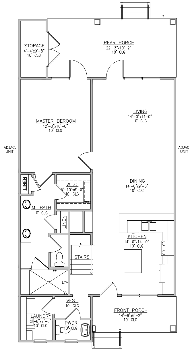
CRANE - 1st FLOOR INTERIOR UNIT
