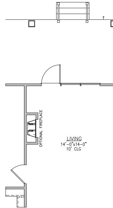
CRANE - 1st FLOOR FIREPLACE OPTION 2
